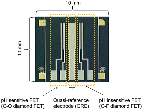
Figure 2 All-solid-state diamond pH sensor under development
