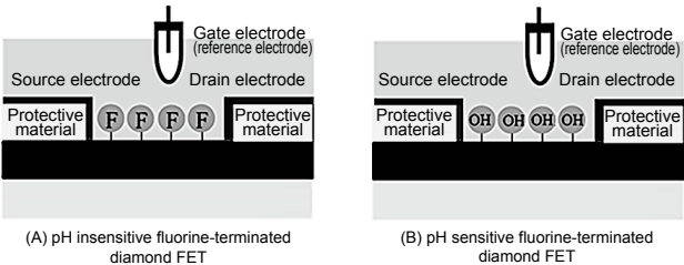
Figure 3 Schematic diagram of surface-modified diamond FET sensor (4)
