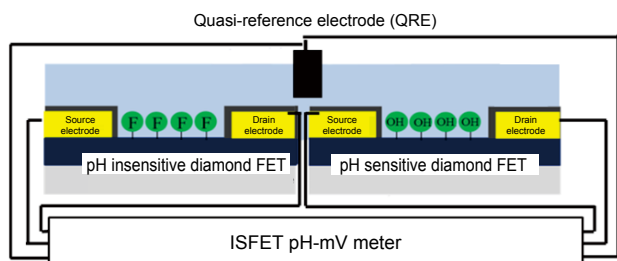
Figure 8 Configuration of the developed all-solid-state pH sensor (4)
