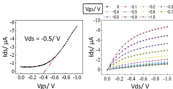
Figure 4 FET current-voltage characteristics of hydrogen-terminated diamond (3)
