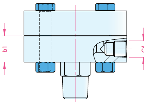
Thickness with flush ports
