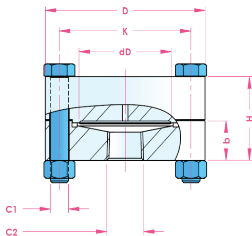
Dimensions table: Female threaded
