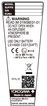
Figure 2.1 Example of Nameplate
