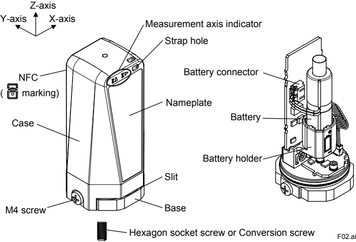
Figure3.1 Component Names
