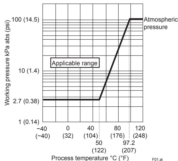
Fig.1 Working Pressure and Process Temperature
