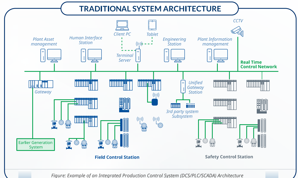
Figure: Example of an Integrated Production Control System (DCS/PLC/SCADA) Architecture
