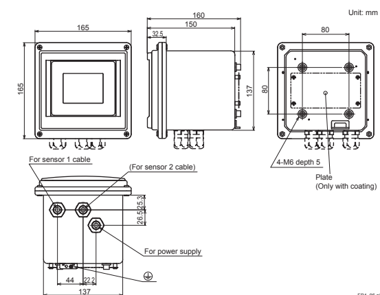
Figure A.10 Housing dimensions and layout of glands (Stainless steel housing)
