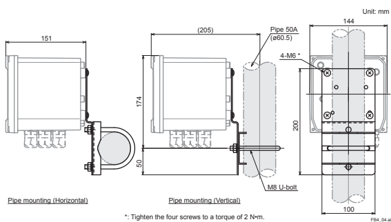
Figure A.7 Pipe mounting (Option /U, /UM) (Plastic housing)
