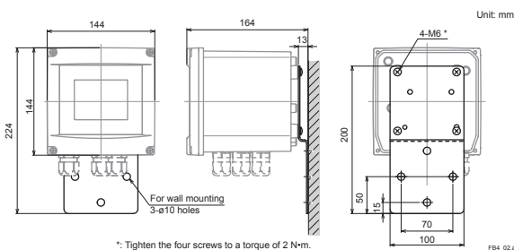
Figure A.6 Wall mounting (Option /U, /UM) (Plastic housing)
