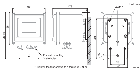
Figure A.12 Wall mounting (Option /U, /UM) (Stainless steel housing)
