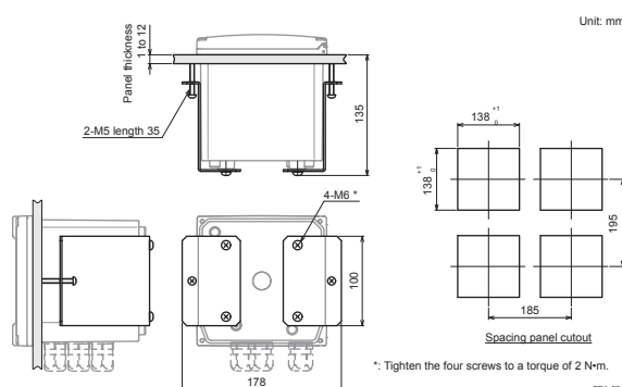
Figure A.5 Panel mounting (Option /PM, /UM) (Plastic housing)
