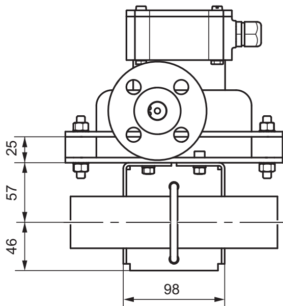
Fig. 23: Dimensions in mm: fixing device option PD for Nano
