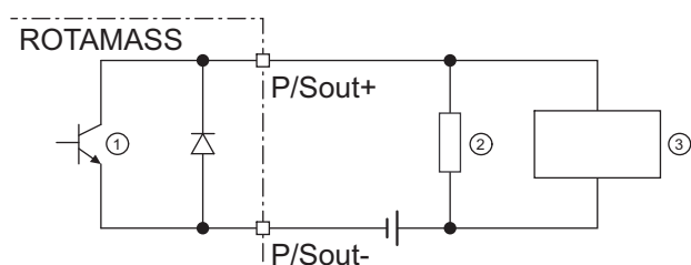
Fig. 35: Passive pulse output connection P/Sout with electronic counter
