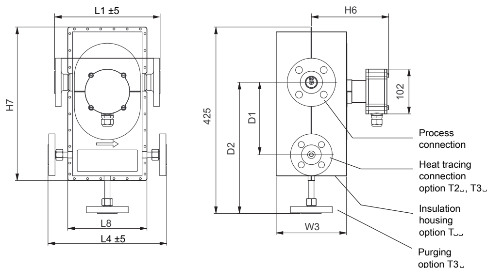
Fig. 24: Dimensions in mm: version with insulation housing
