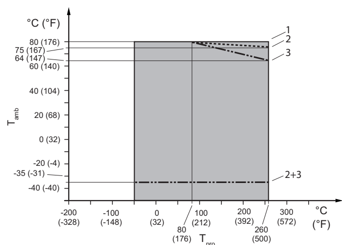
Fig. 20: Allowed process fluid and ambient temperatures
