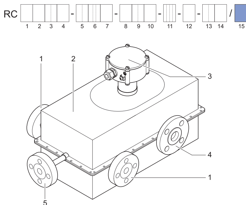
Fig. 17: Configuration of Rotamass with insulation and heat tracing
