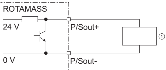
Fig. 38: Active status output P/Sout with internal pull-up resistor
