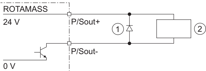
Fig. 33: Active pulse output P/Sout connection with electromechanical counter
