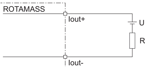
Fig. 29: Passive current output connection I out
