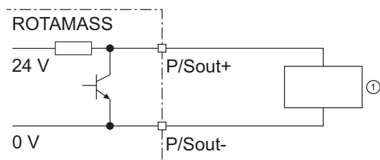
Fig. 34: Active pulse output P/Sout with internal pull-up resistor
