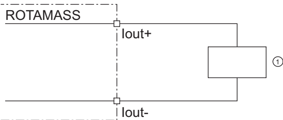
Fig. 27: Active current output connection Iout HART
