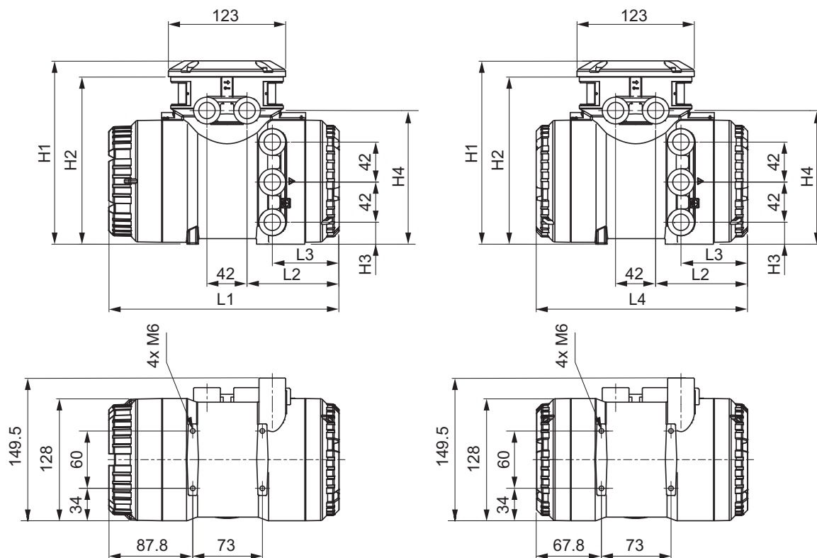
Fig. 25: Dimensions of transmitter in mm (left: transmitter with display, right: transmitter without display)
