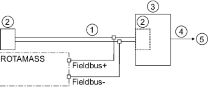
Fig. 43: PROFIBUS PA connection
