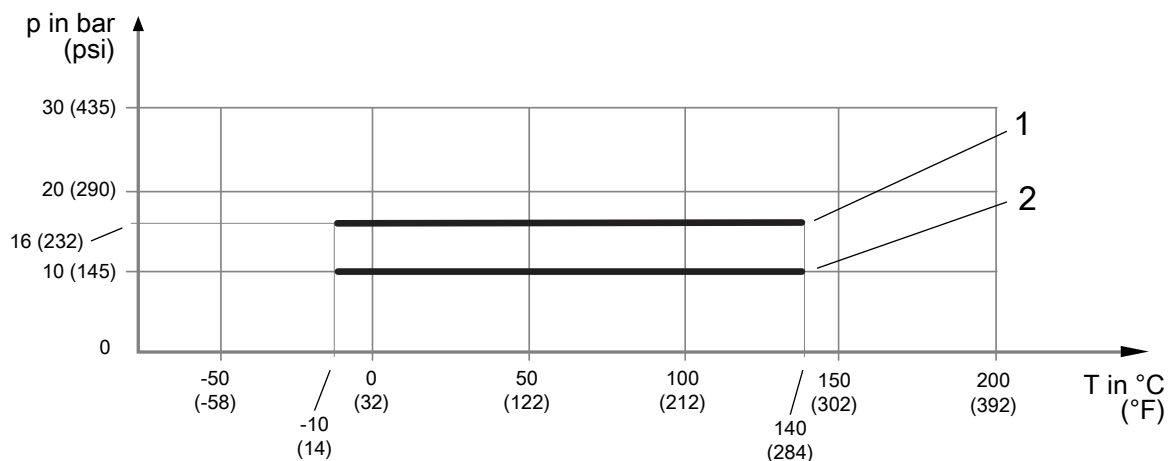
Fig. 14: Allowed process pressure as a function of process fluid temperature
