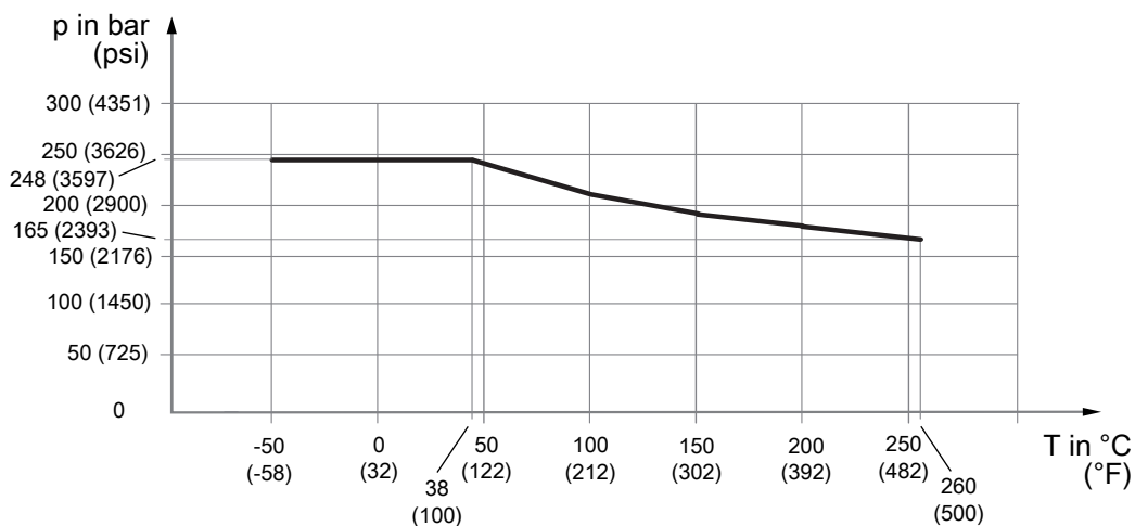
Fig. 11: Allowed process pressure as a function of process connection temperature
