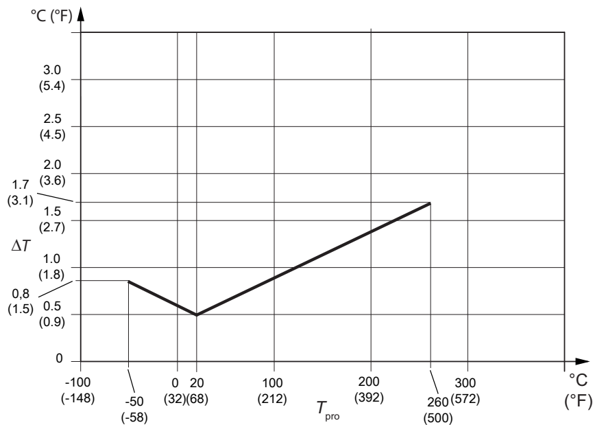
Fig. 5: Temperature accuracy
