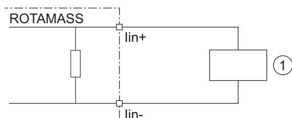
Fig. 31: Connection of external device with active current output
