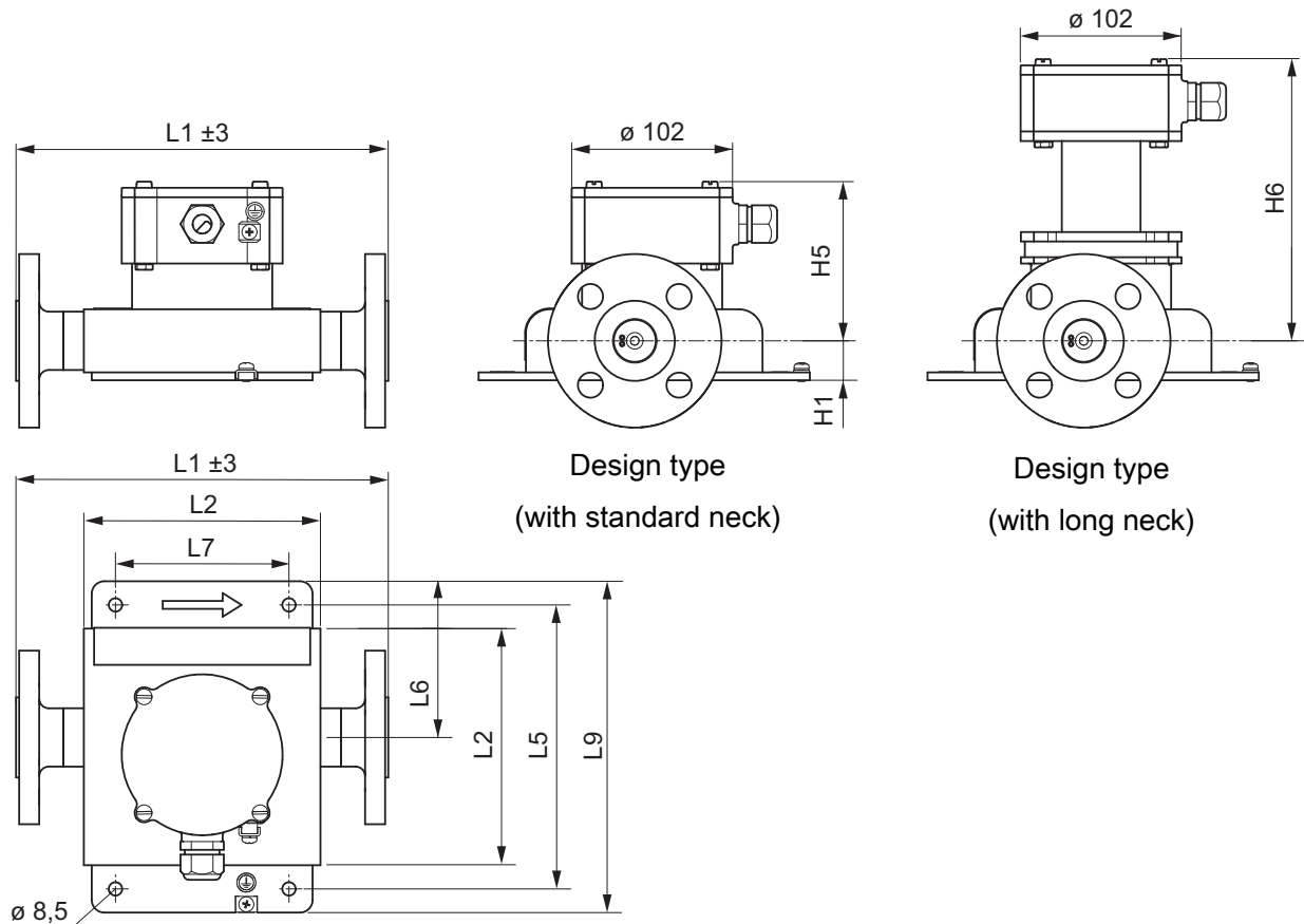
Fig. 22: Dimensions in mm
