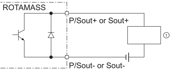
Fig. 39: Passive status output connection P/Sout or Sout
