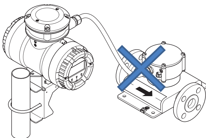
Fig. 6: Installation position to be avoided: Flow meter in sideways position
