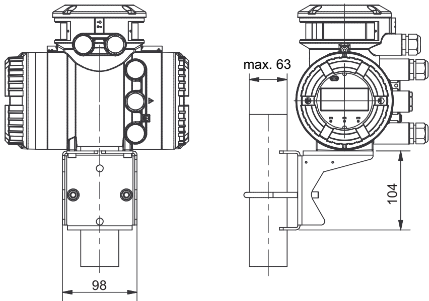
Fig. 26: Dimensions of transmitter in mm, attached to mounting bracket.
