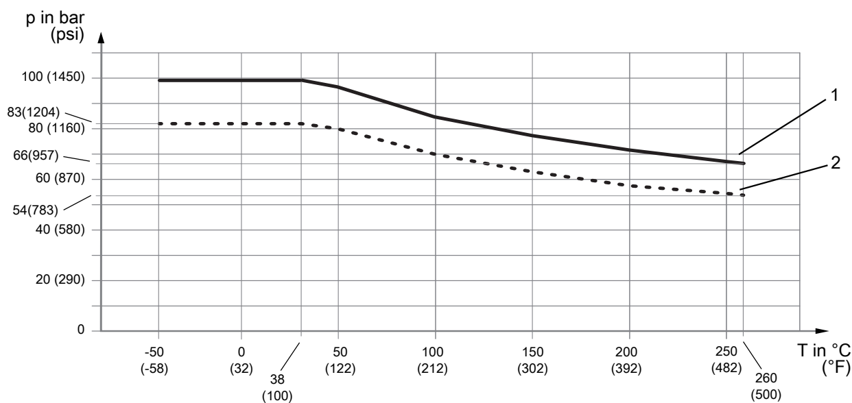
Fig. 9: Allowed process pressure as a function of process connection temperature
