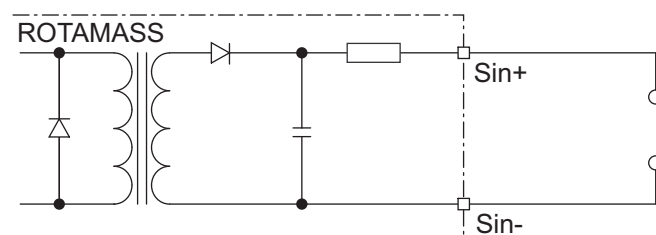
Fig. 42: Status input connection
