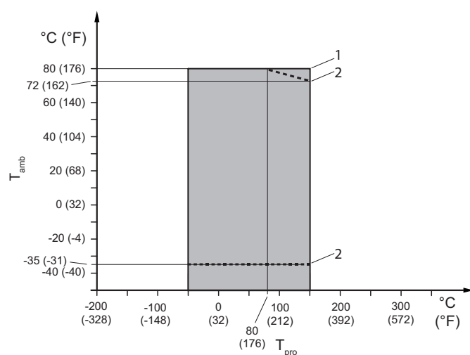
Fig. 18: Allowed process fluid and ambient temperatures, remote type (except process connection type HS4 and HS8)
