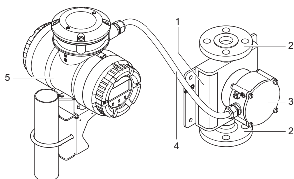
Fig. 2: Configuration of the Rotamass remote type
