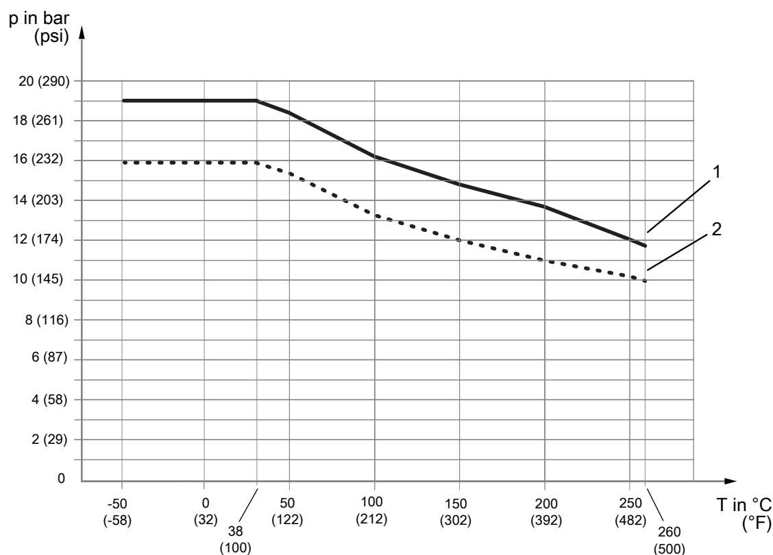
Fig. 7: Allowed process pressure as a function of process connection temperature
