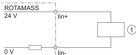
Fig. 30: Connection of external device with passive current output
