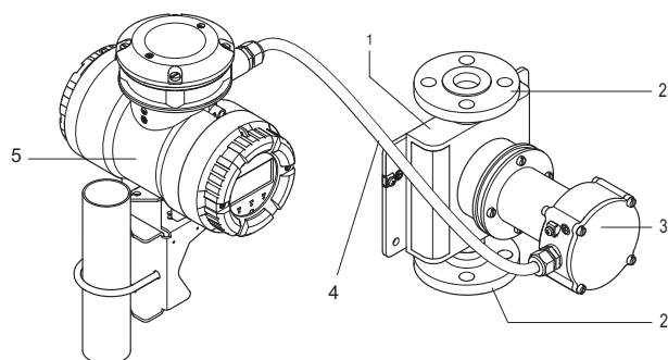
Fig. 3: Configuration of the Rotamass remote type - long neck
