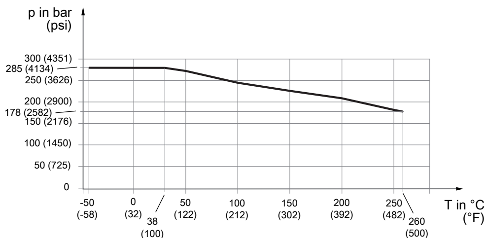
Fig. 16: Allowed process pressure as a function of process fluid temperature
