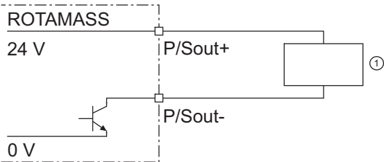
Fig. 37: Active status output connection P/Sout
