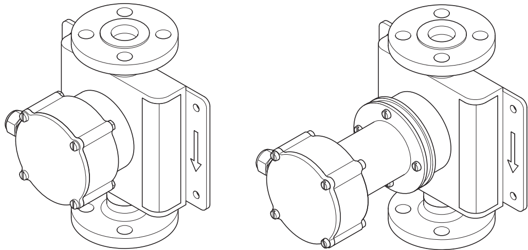
Fig. 21: Sensor with standard and long neck
