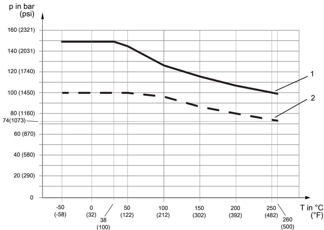
Fig. 10: Allowed process pressure as a function of process connection temperature
