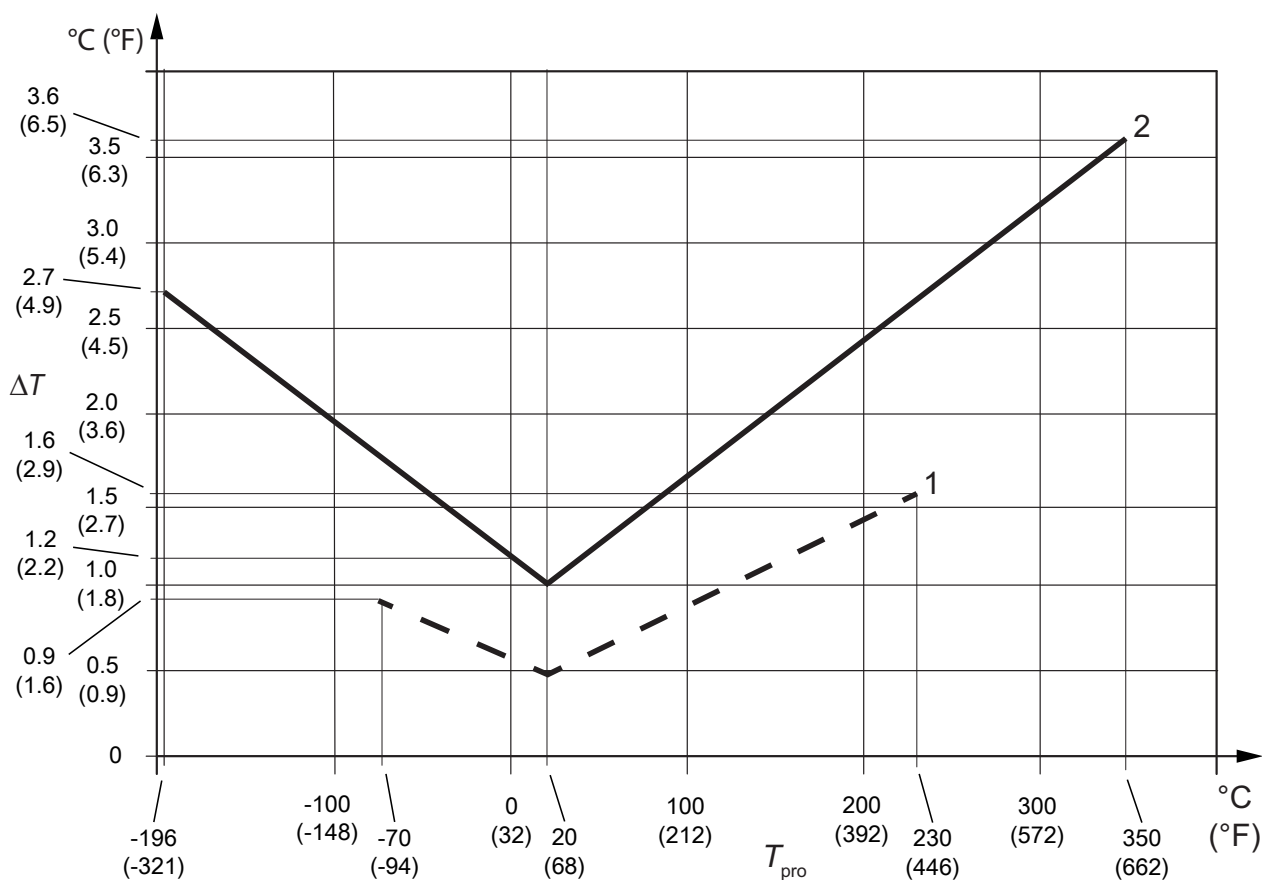
Fig. 6: Presentation of temperature accuracy
