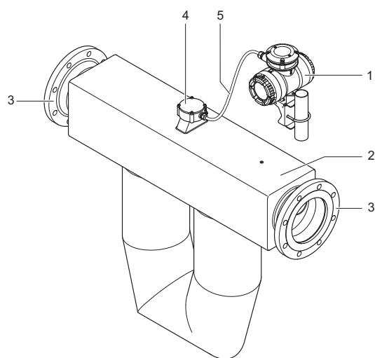
Fig. 3: Configuration of the Rotamass remote type
