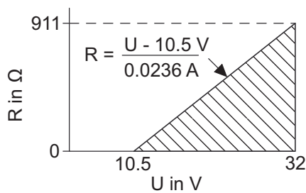
Fig. 19: Maximum load resistance as a function of an external power supply voltage
