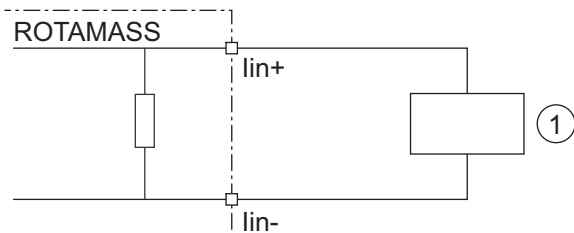
Fig. 22: Connection of external device with active current output
