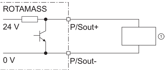
Fig. 29: Active status output P/Sout with internal pull-up resistor
