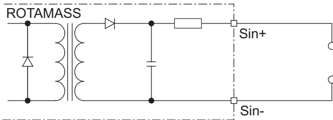
Fig. 33: Status input connection
