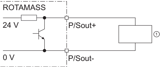
Fig. 25: Active pulse output P/Sout with internal pull-up resistor
