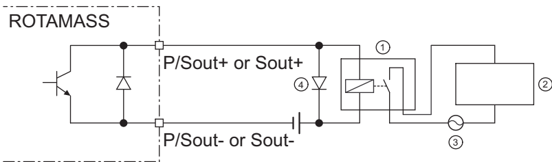
Fig. 31: Passive status output connection P/Sout or Sout for solenoid valve circuit
