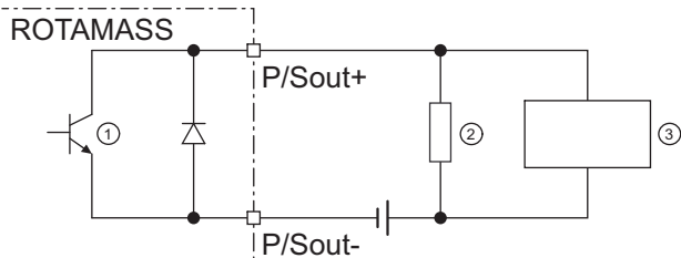
Fig. 26: Passive pulse output connection P/Sout with electronic counter
