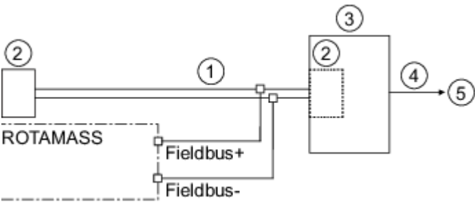
Fig. 34: PROFIBUS PA connection
