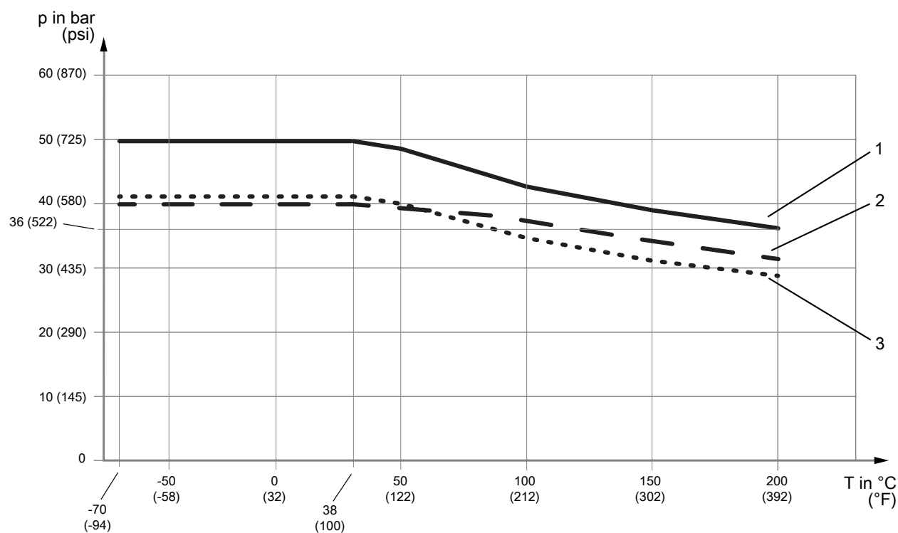
Fig. 8: Allowed process pressure as a function of process fluid temperature
