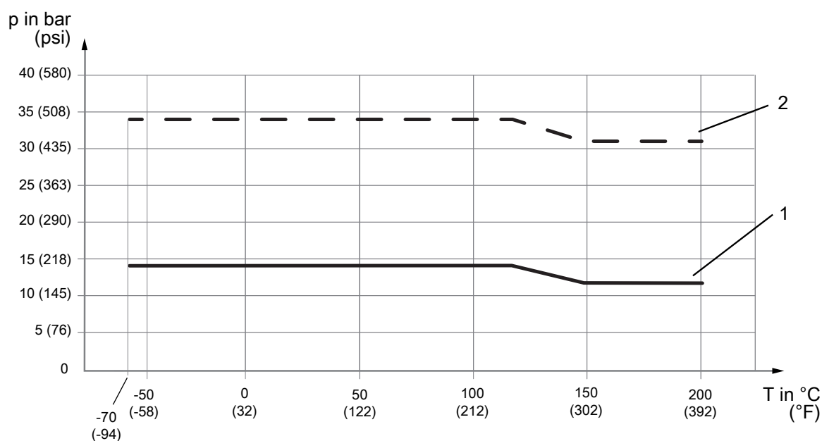
Fig. 11: Allowed process pressure as a function of process fluid temperature
