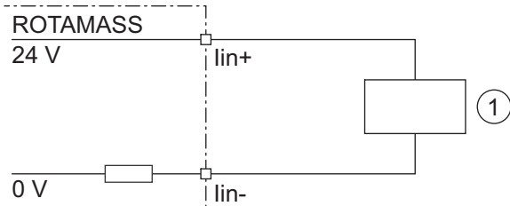
Fig. 21: Connection of external device with passive current output
