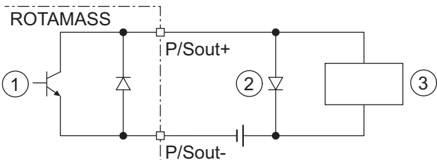
Fig. 27: Passive pulse output P/Sout connection with electromechanical counter
