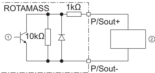
Fig. 32: Passive pulse or status output with switching amplifier connected in series
