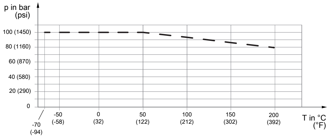
Fig. 10: Allowed process pressure as a function of process fluid temperature, compatible to flange EN 1092-1 PN100
