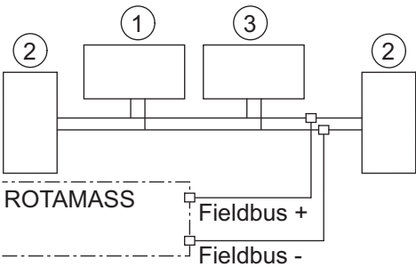
Fig. 35: FOUNDATION Fieldbus connection
