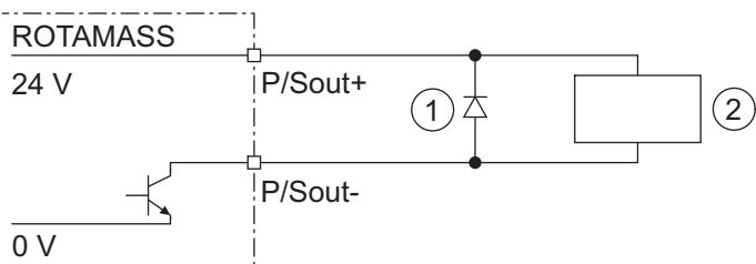
Fig. 24: Active pulse output P/Sout connection with electromechanical counter
