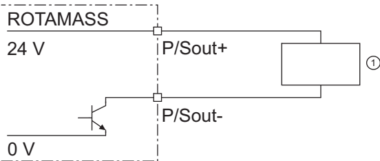
Fig. 28: Active status output connection P/Sout
