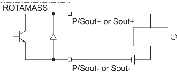
Fig. 30: Passive status output connection P/Sout or Sout
