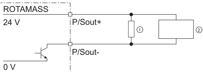
Fig. 23: Active pulse output connection P/Sout
