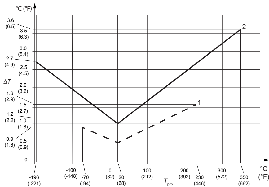
Fig. 6: Temperature accuracy
