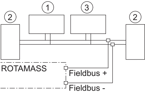
Fig. 38: FOUNDATION Fieldbus connection
