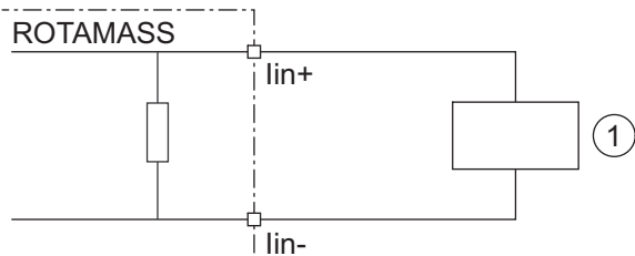
Fig. 25: Connection of external device with active current output
