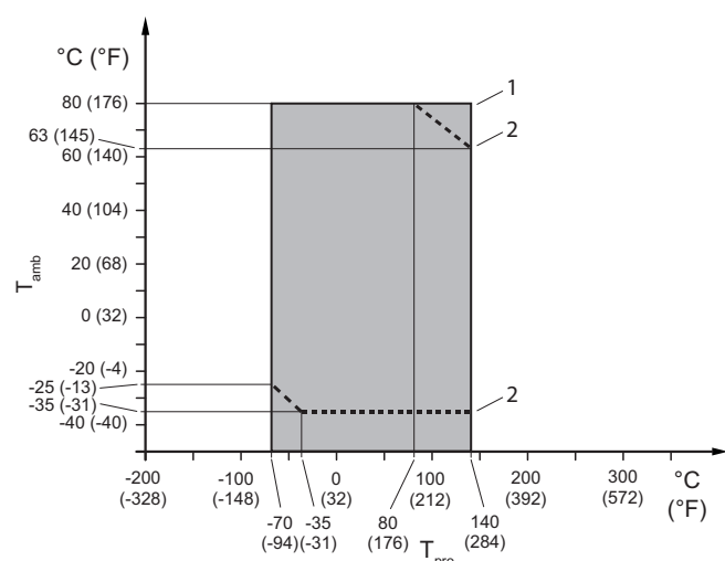
Fig. 15: Allowed process fluid and ambient temperatures, remote type for process connection type HS2, HS6 and HS9
