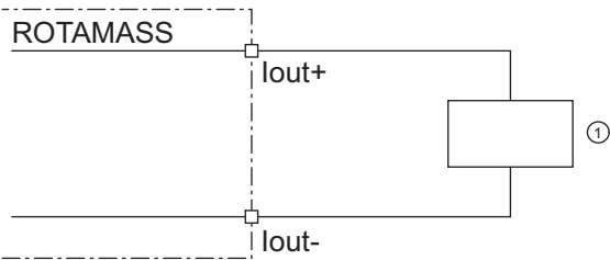
Fig. 21: Active current output connection lout HART
