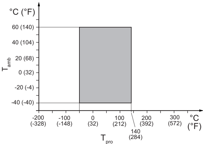
Fig. 13: Allowed process fluid and ambient temperatures, integral type for process connection type HS2, HS3, HS6 and HS9
