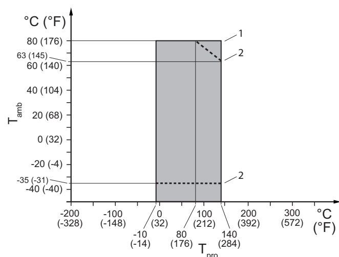
Fig. 16: Allowed process fluid and ambient temperatures, remote type for process connection type HS4 and HS8
