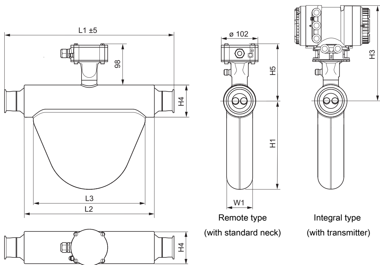
Fig. 19: Dimensions in mm
