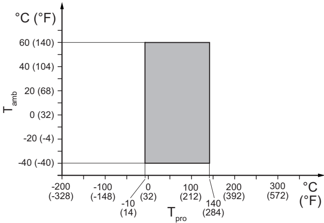
Fig. 14: Allowed process fluid and ambient temperatures, integral type for process connection type HS4 and HS8
