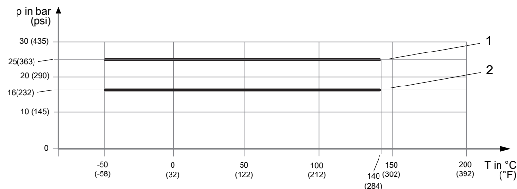
Fig. 11: Allowed process pressure as a function of process fluid temperature
