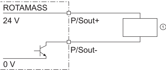
Fig. 31: Active status output connection P/Sout
