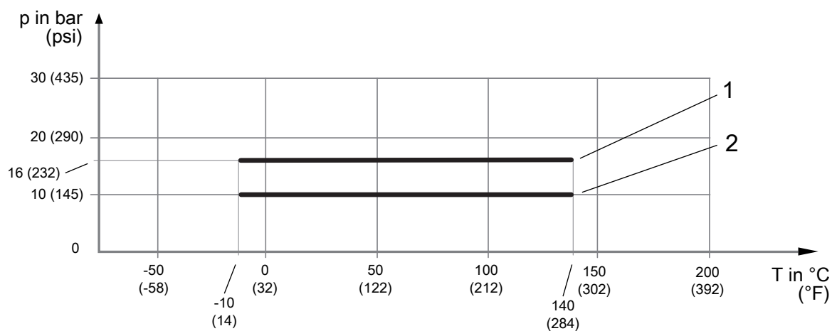
Fig. 10: Allowed process pressure as a function of process fluid temperature
