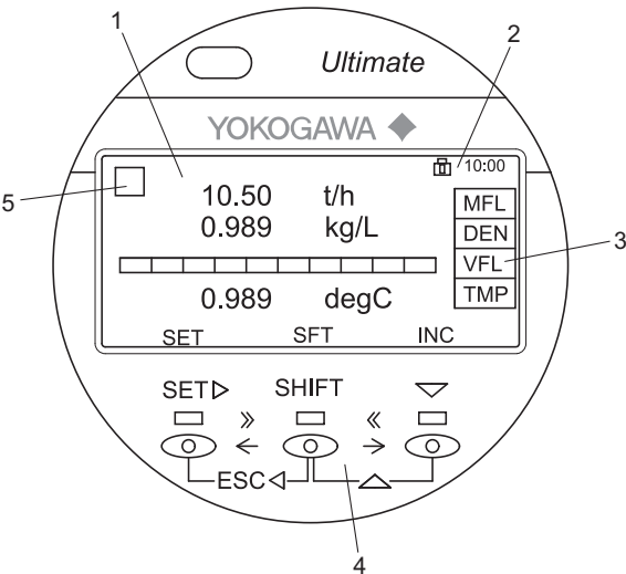
Fig. 40: Display layout
