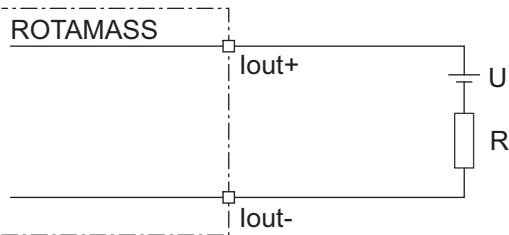
Fig. 23: Passive current output connection I out
