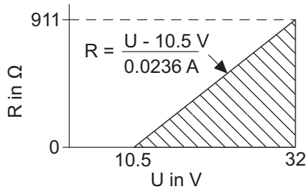
Fig. 22: Maximum load resistance as a function of an external power supply voltage
