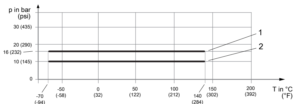
Fig. 12: Allowed process pressure as a function of process connection temperature
