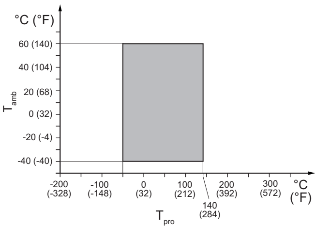
Fig. 17: Allowed process fluid and ambient temperatures, remote type for process connection type HS3
