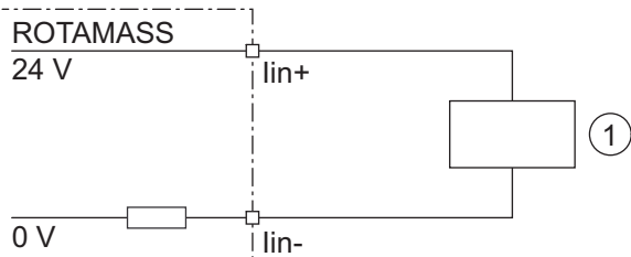
Fig. 24: Connection of external device with passive current output
