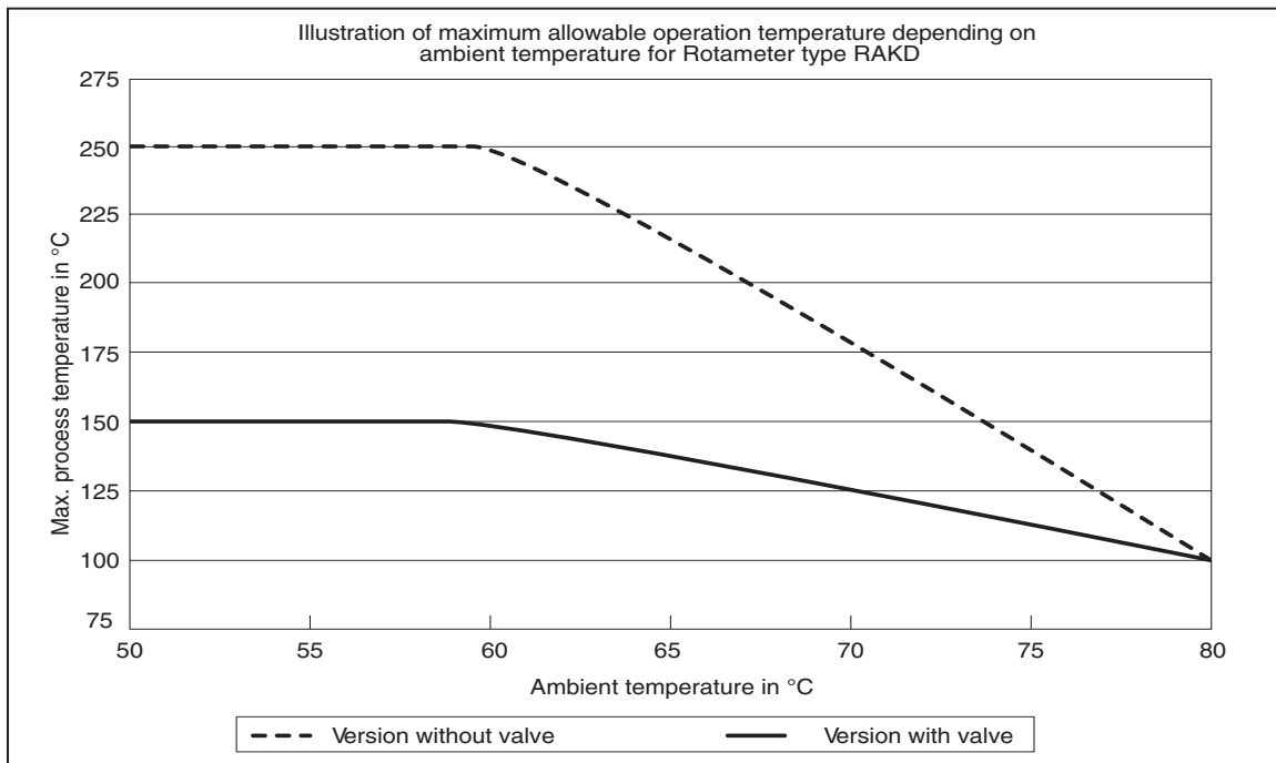
Fig. 2-1 Temperature specification
