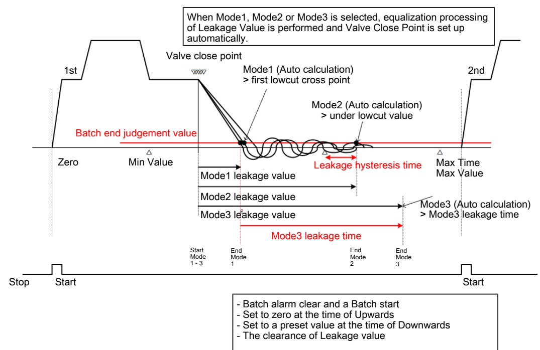
Fig. 17: Leakage compensation mode
