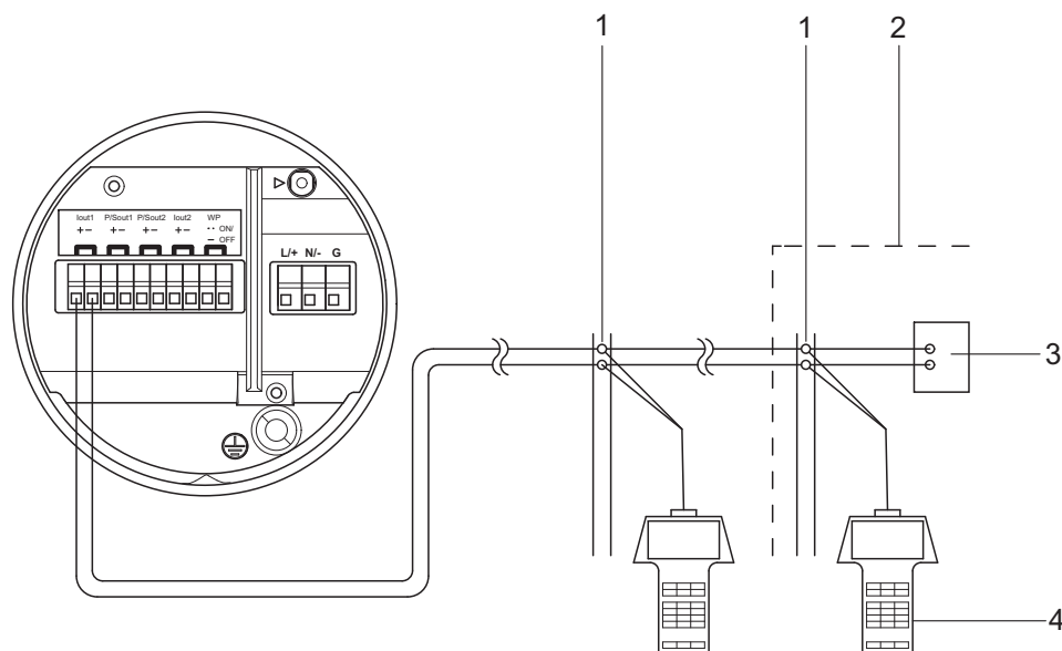
Fig. 1: Connection diagram HART field communicator
