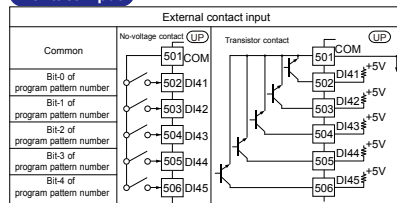
Contact rating: 12 V DC, 10 mA or more
