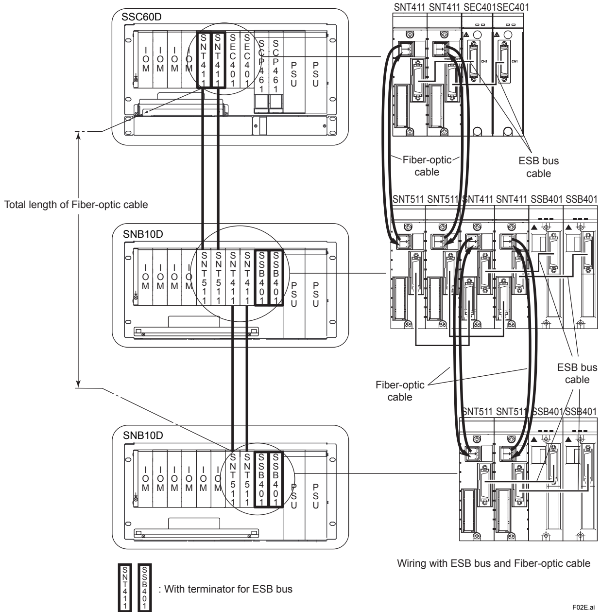
Figure Example of Chain Type Connection
