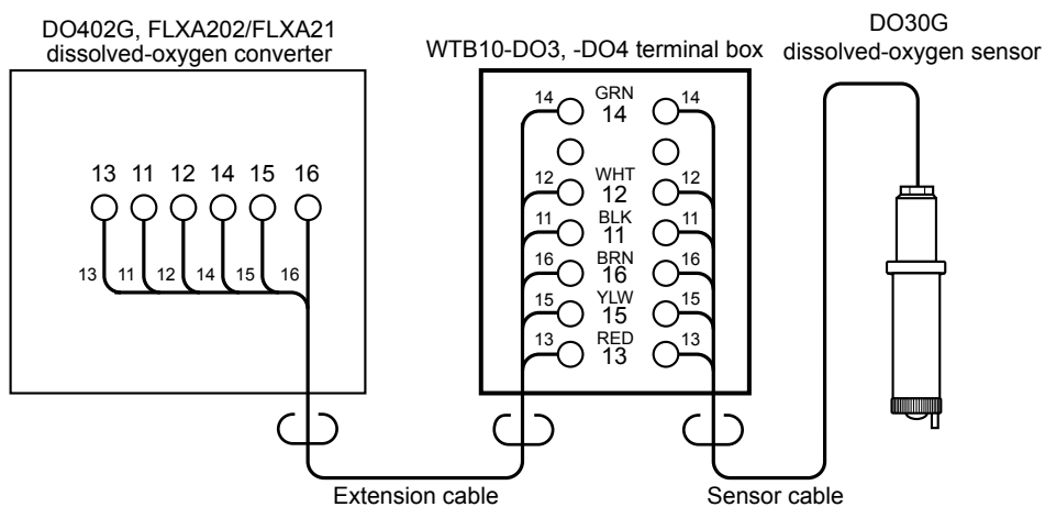
Figure 2.6 Wire Connections to WTB10-DO3, -DO4 Terminal Box
