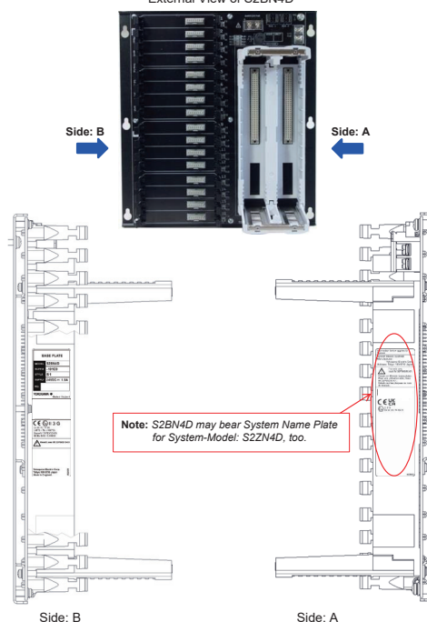
External View of S2BN4D
