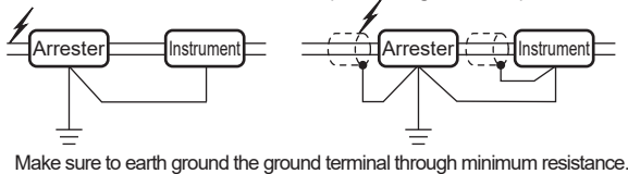
(1) Interconnect Grounding (2) Interconnect Grounding (when using shield line)
