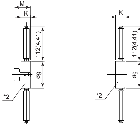
Straight type (raised face) Reducer type (raised face)
