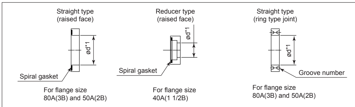
Straight type (raised face) Reducer type (raised face)
