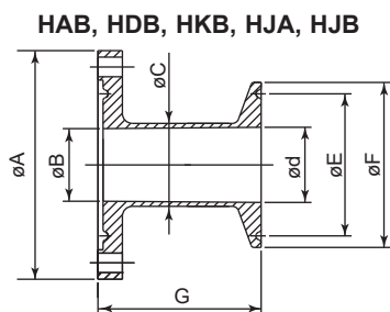
Clamp Connection Adapter
