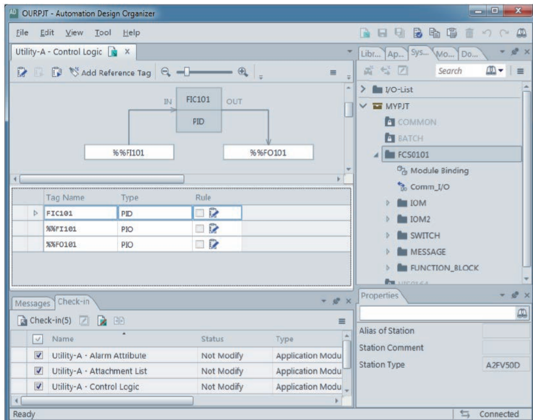
Figure AD Organizer
