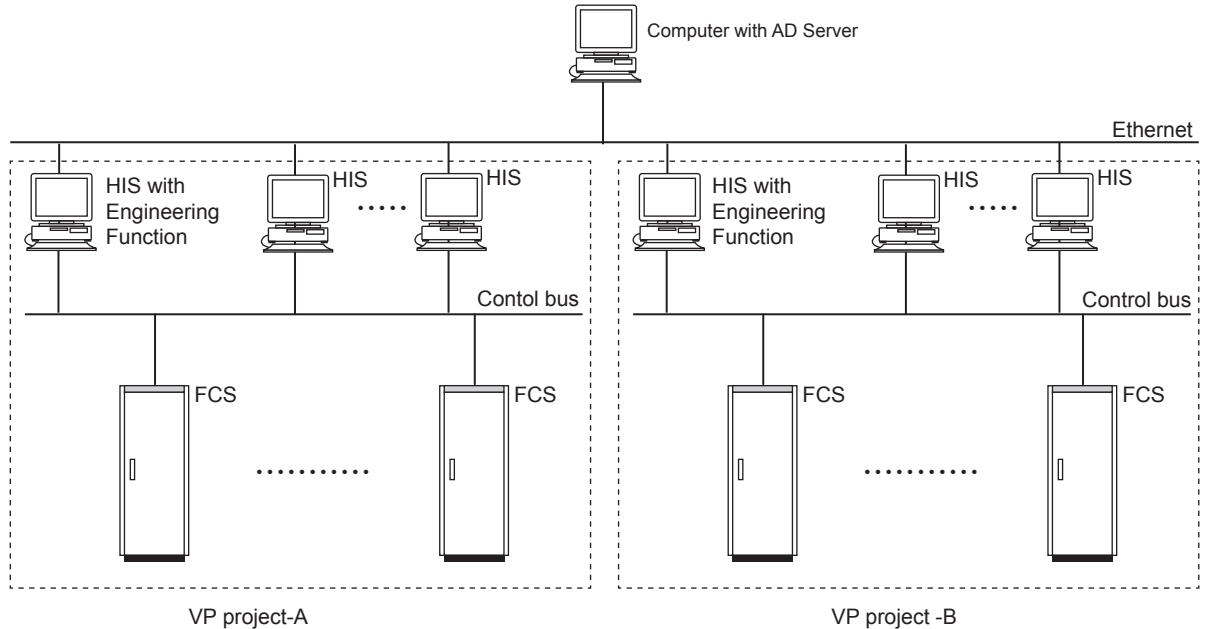
Figure A sample system configuration to collectively manage multiple VP Projects
