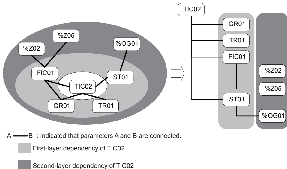
Figure Conceptual Diagram Displaying Dependency (Control Logic Dependency)
