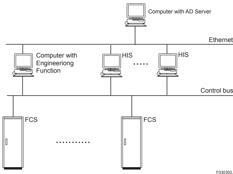
Figure A sample system configuration where Engineering Function of AD Server and Operation and Monitoring Function are installed on separate computers
