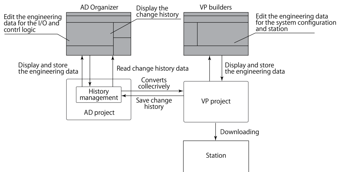
Figure Engineering Data Flow of Module-based Engineering
