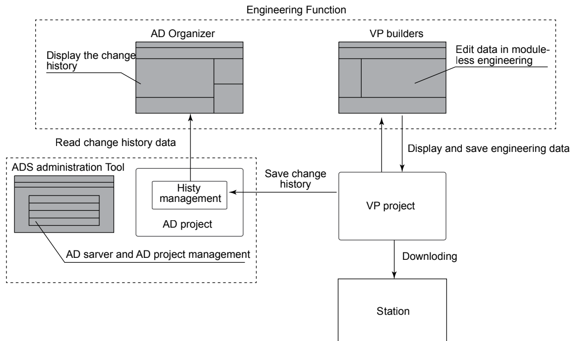
Figure Engineering Data Flow of the Standard Function of AD Suite
