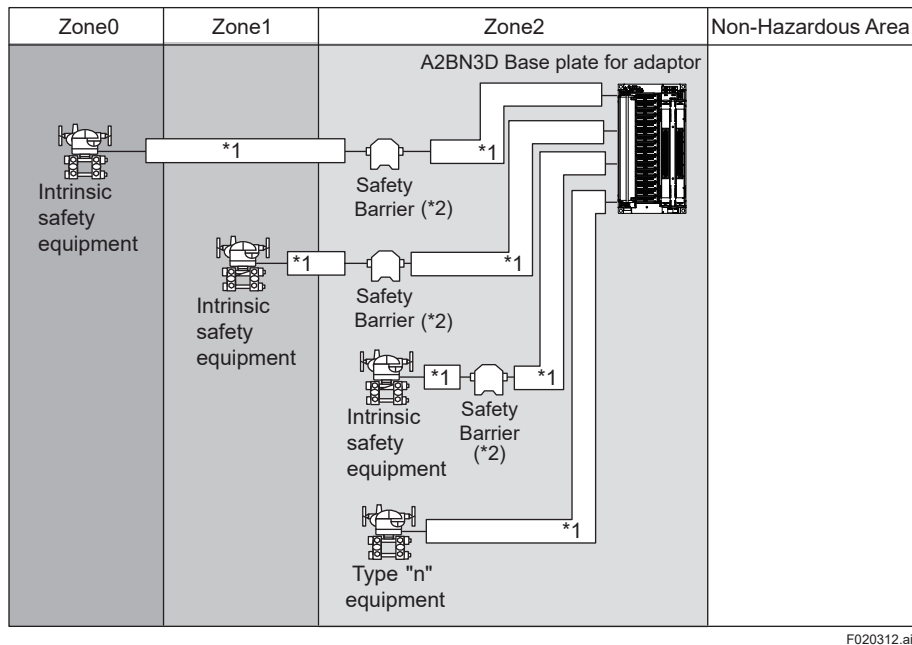
Figure Connection of A2BN3D for ATEX and IECEx (2)
