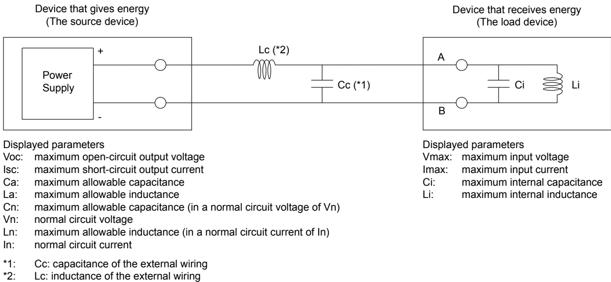
Figure Connection of CSA NI Devices and Associated Parameters
