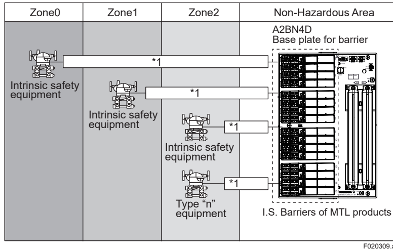
Figure Connection of A2BN4D for ATEX and IECEx (1)
