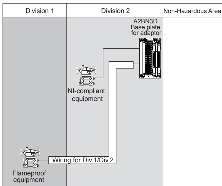
Figure Connection of A2BN3D for FM and CSA (2)
