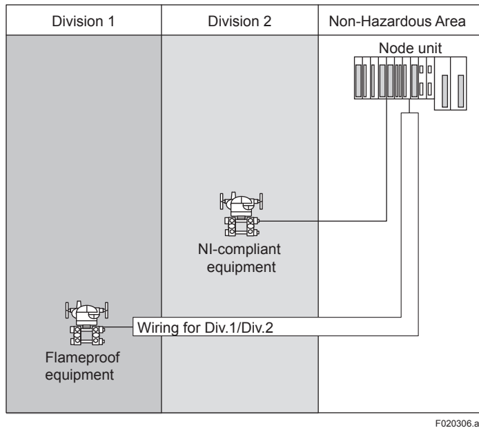
Figure Connection of an NI Compliant Module (1)
