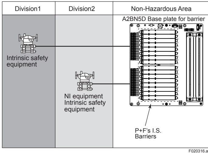
Figure Connection of A2BN5D for FM and CSA (1)
