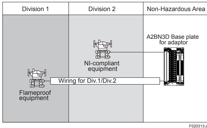
Figure Connection of A2BN3D for FM and CSA (1)
