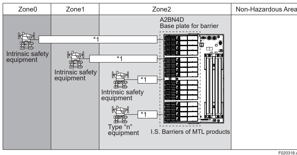
Figure Connection of A2BN4D for ATEX and IECEx (2)
