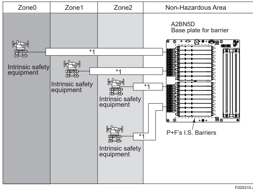
Figure Connection of A2BN5D for ATEX and IECEx (1)
