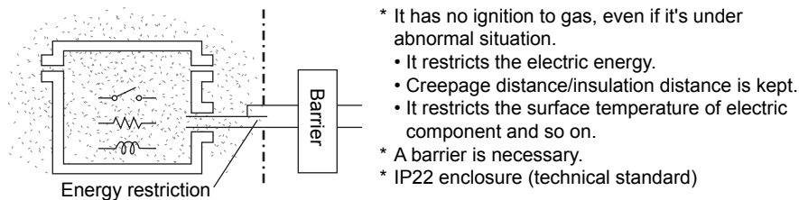
Figure Intrinsic Safety (Type “i”)
