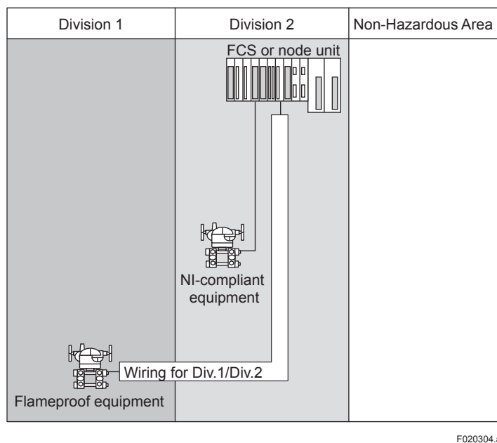
Figure Connection of an NI Compliant Module (2)
