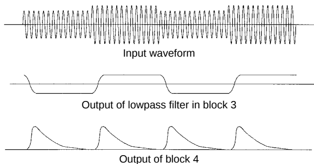
Figure 5 Output Waveforms
