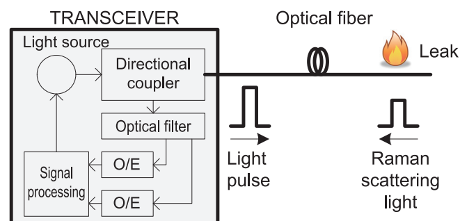
Figure 2. A light pulse is generated by the transceiver, and the intensity of the Raman scattering light is measured by the transceiver, pinpointing temperature changes along the length of the fibre optic cable.
